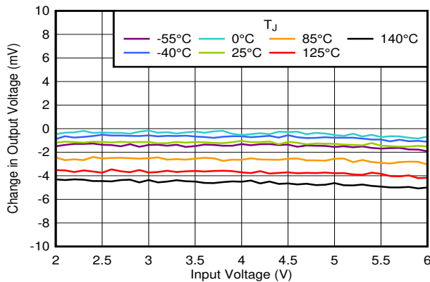
Figure 6-25. Line Regulation vs V_{IN} and Temperature
